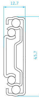
NJ-3D ( 100lb / 45Kgs )
