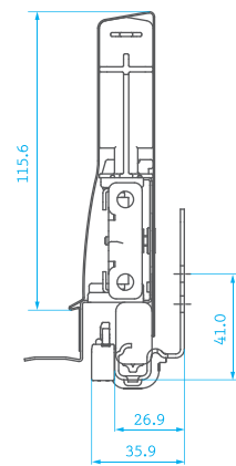
NJ-A5802 ( 75lb / 35Kgs )
