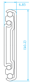
NJ-2J ( 75lb / 35Kgs )
