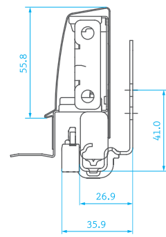
NJ-A5801 ( 75lb / 35Kgs )
