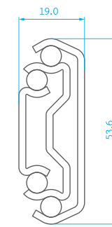
NJ-7000 ( 200lb / 90Kgs )
