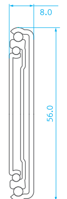
NJ-2D ( 176lb / 80Kgs )
